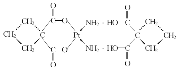
Fig 1. The chemical structure of 0325k_{1-1}
