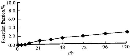
Fig 5. The cumulated excretion of 0325k 1-1 in rat faeces after iv injection
