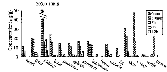
Fig 3. Tissue concentration of 0325k 1-1 in the rats at different time after iv injection
