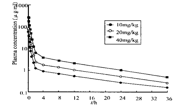
Fig 2. Plasma concentration-time profiles of 0325k 1-1 in the rats after iv injection
