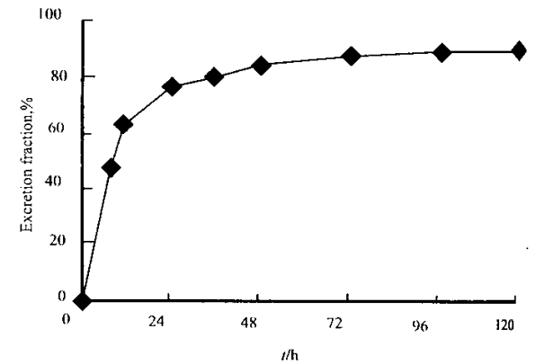
Fig 4. The cumulated excretion of 0325k 1-1 in rat urine after iv injection
